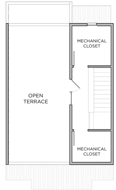
FOURTH FLOOR
